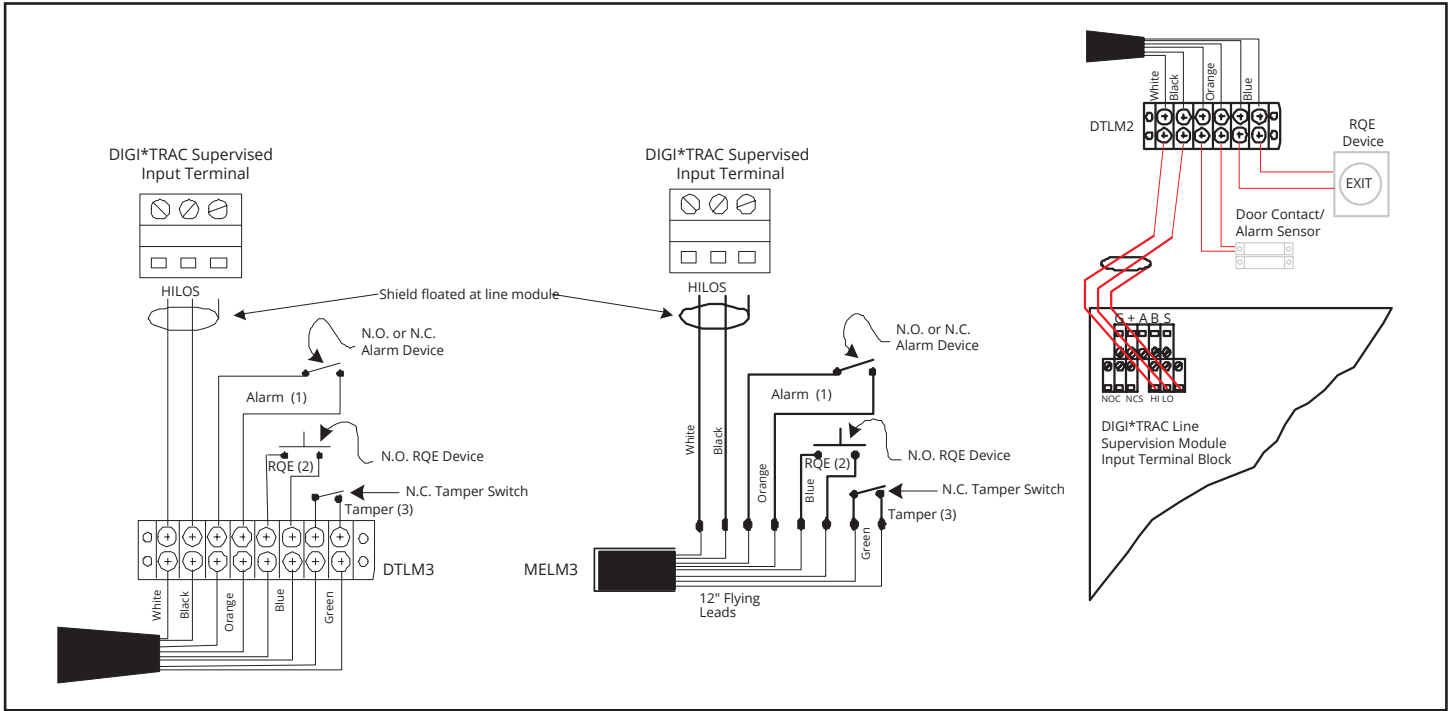
Figure 1: Typical Controller-to-Line Module Wiring Diagram
